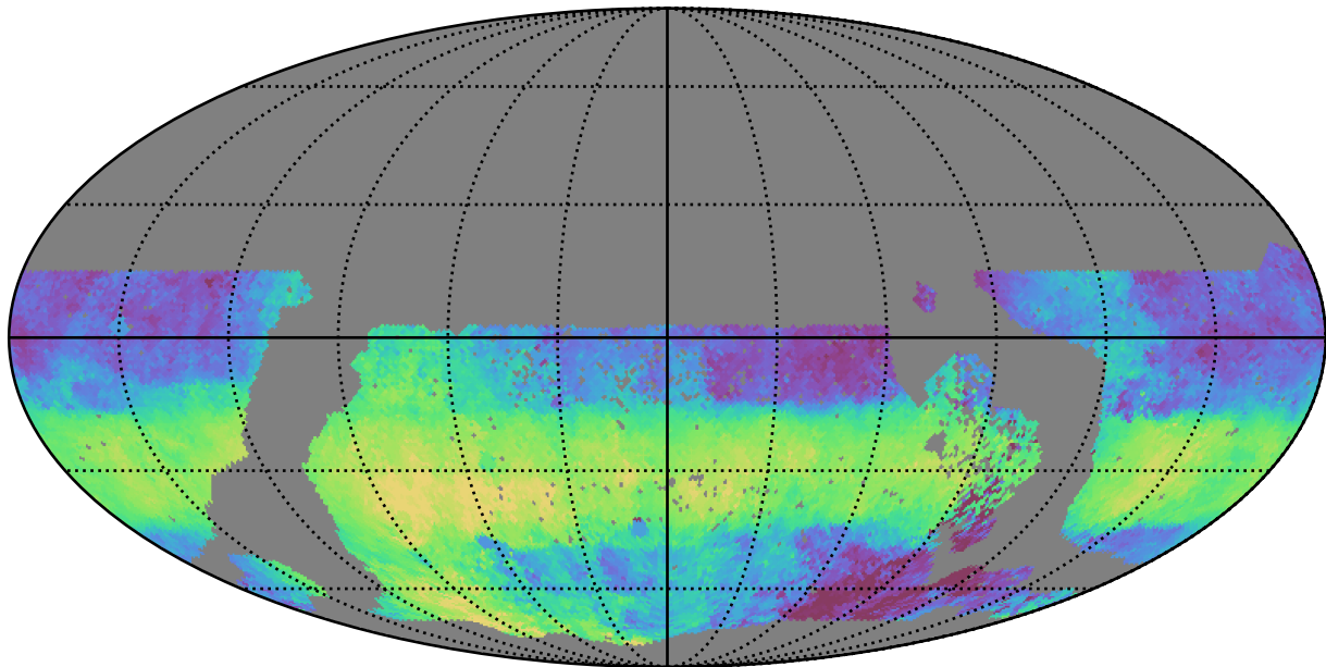
too_elab_r32_d3_ugrizy_v3.4_10yrs WFD u band: Median HA
