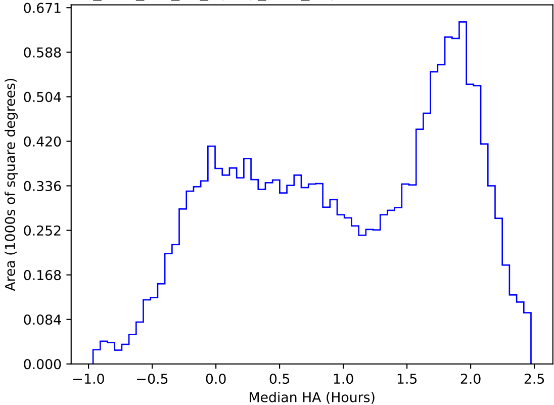
too_elab_r32_d3_ugrizy_v3.4_10yrs WFD u band: Median HA
