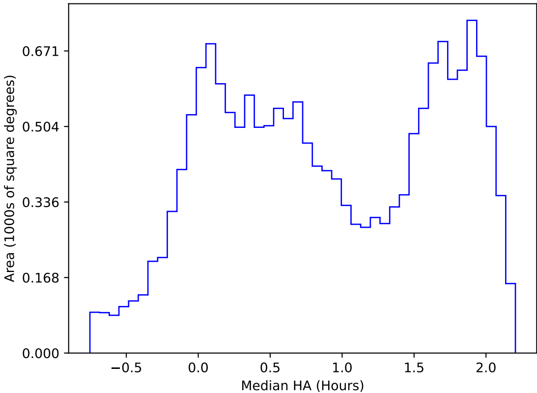
too_elab_r32_d3_ugrizy_v3.4_10yrs WFD r band: Median HA
