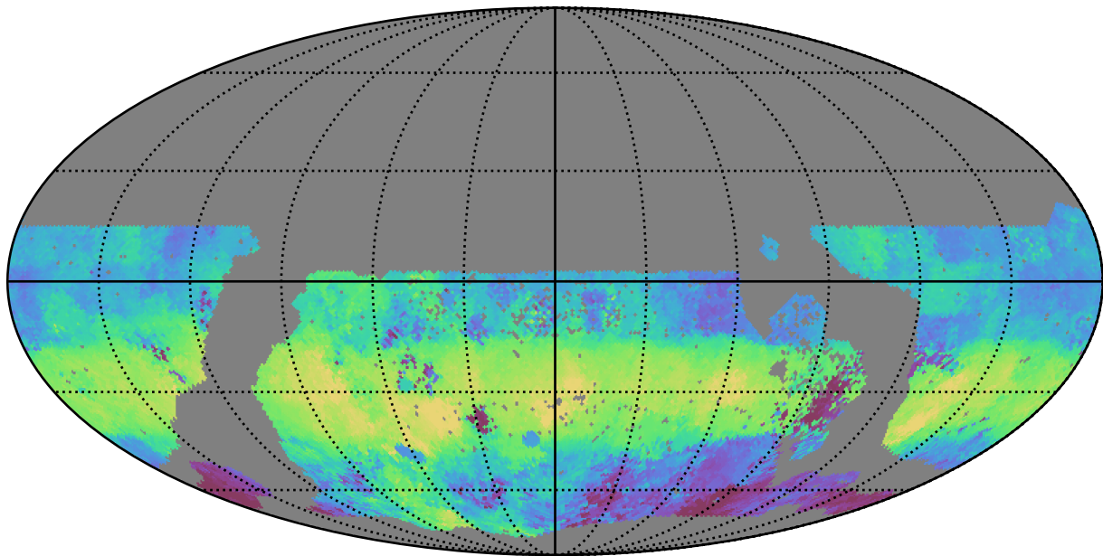
too_elab_r32_d3_ugrizy_v3.4_10yrs WFD g band: Median HA
