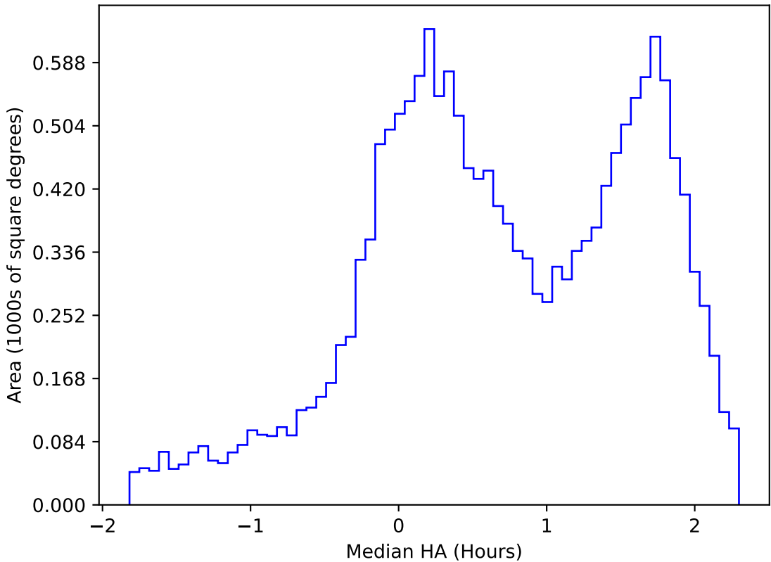
too_elab_r32_d3_ugrizy_v3.4_10yrs WFD g band: Median HA
