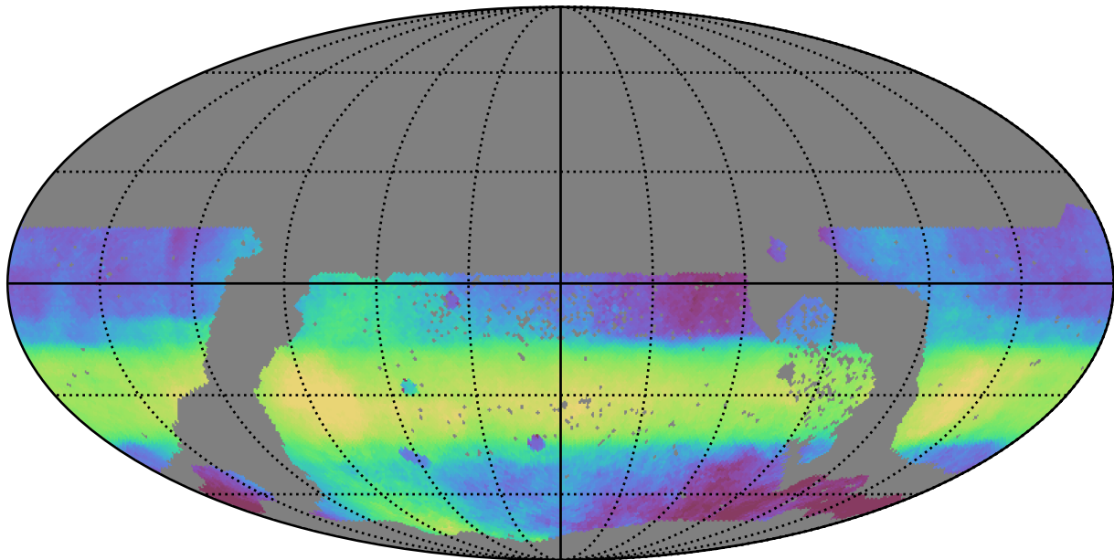
too_elab_r32_d3_ugrizy_v3.4_10yrs WFD all bands: Median HA
