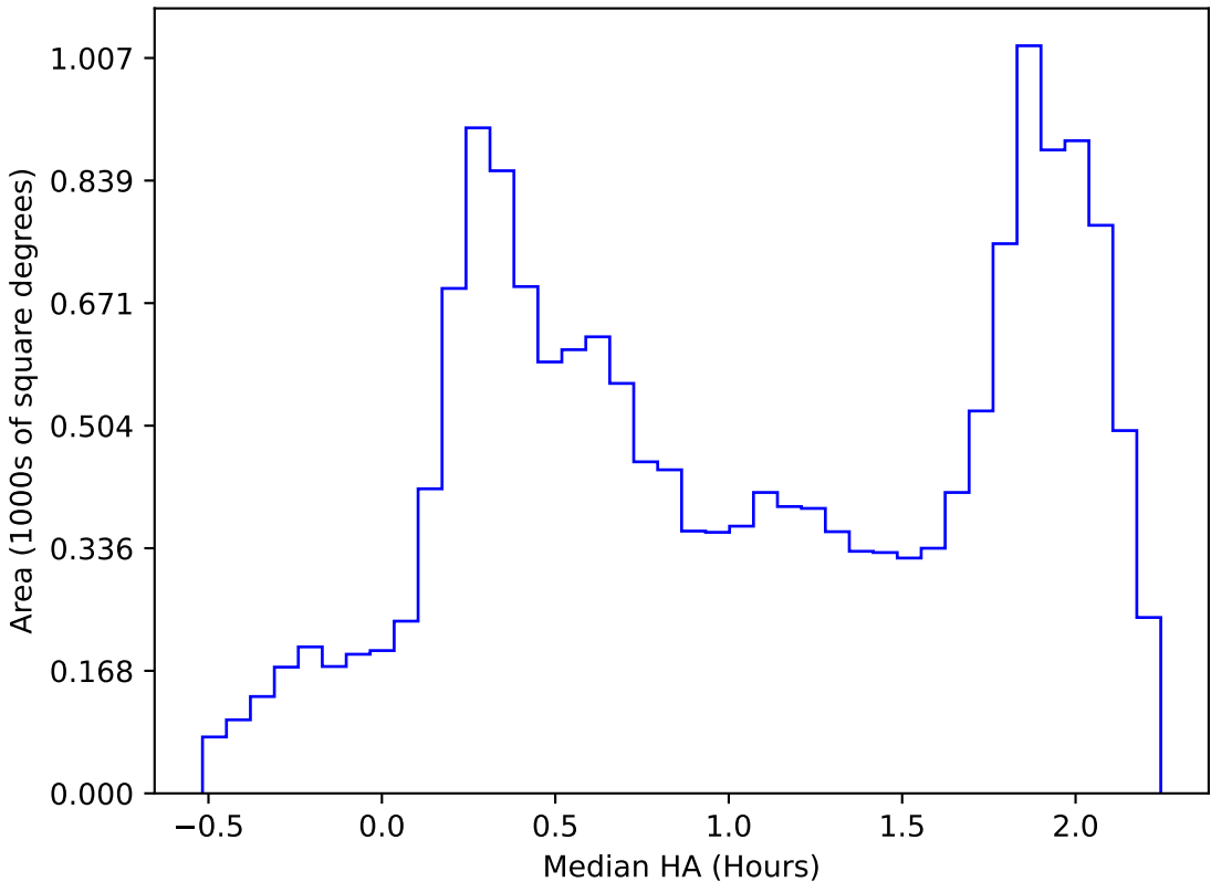
too_elab_r32_d3_ugrizy_v3.4_10yrs WFD all bands: Median HA
