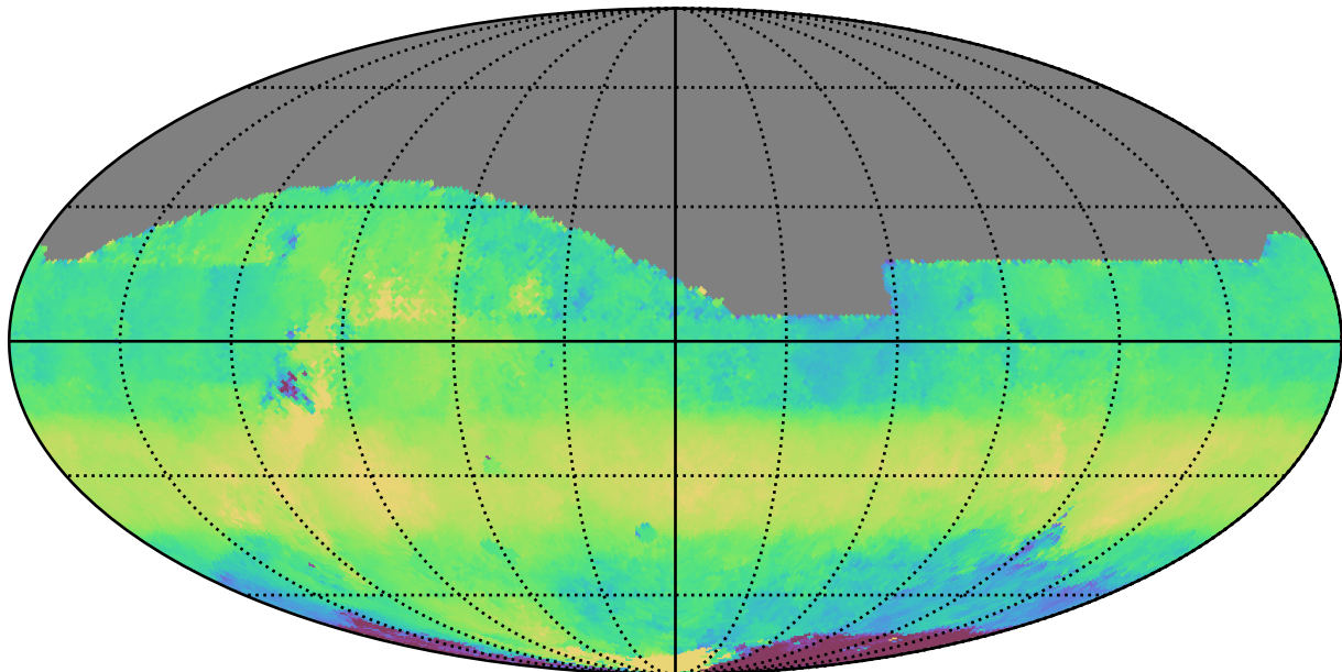
too_elab_r32_d3_ugrizy_v3.4_10yrs All sky z band: Median HA
