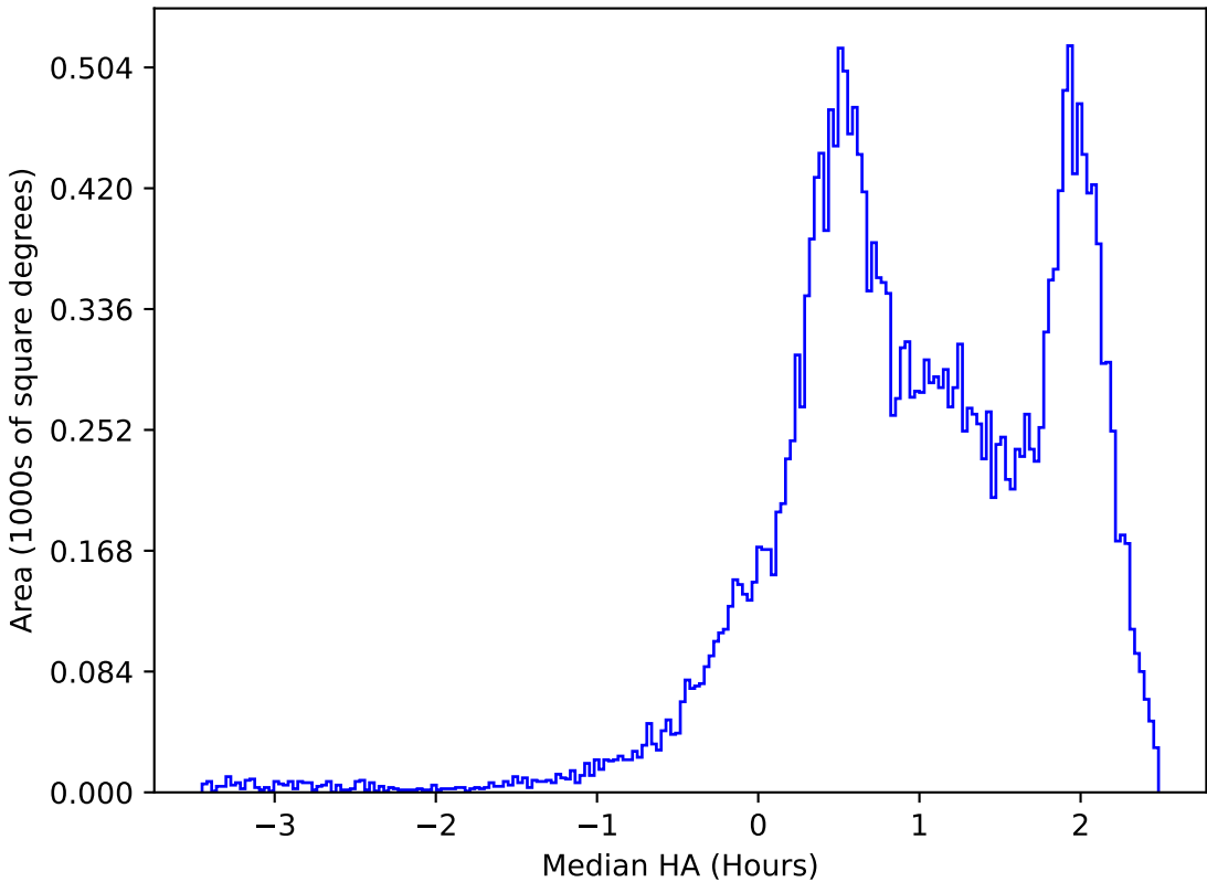
too_elab_r32_d3_ugrizy_v3.4_10yrs All sky z band: Median HA
