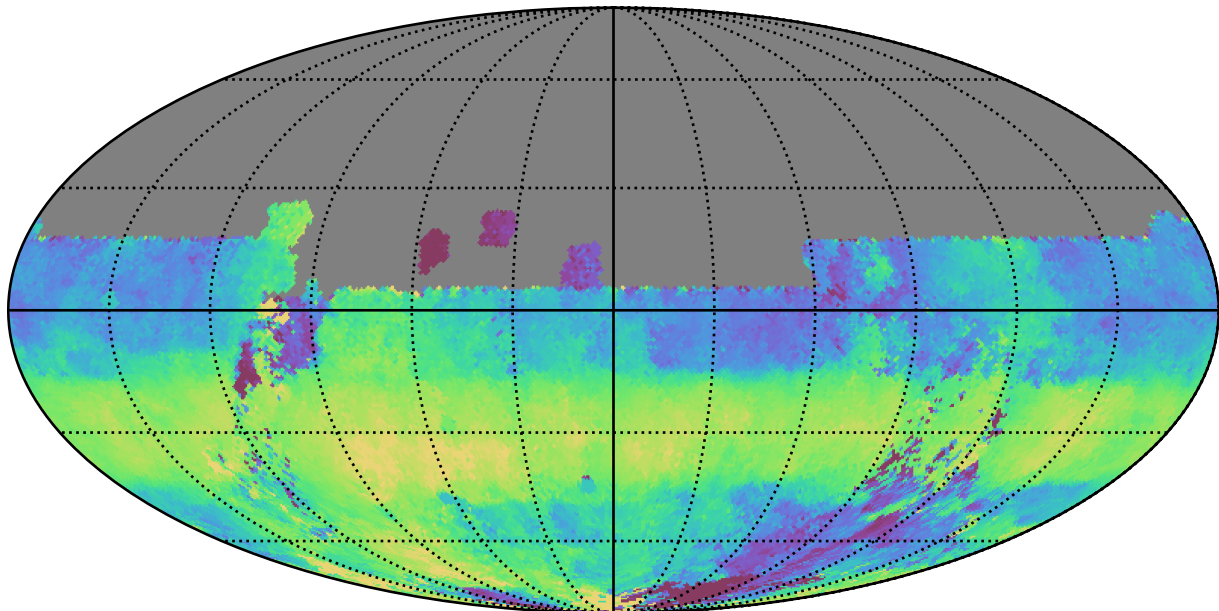
too_elab_r32_d3_ugrizy_v3.4_10yrs All sky u band: Median HA
