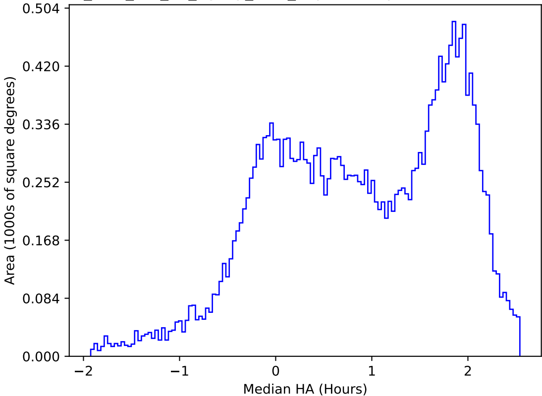
too_elab_r32_d3_ugrizy_v3.4_10yrs All sky u band: Median HA
