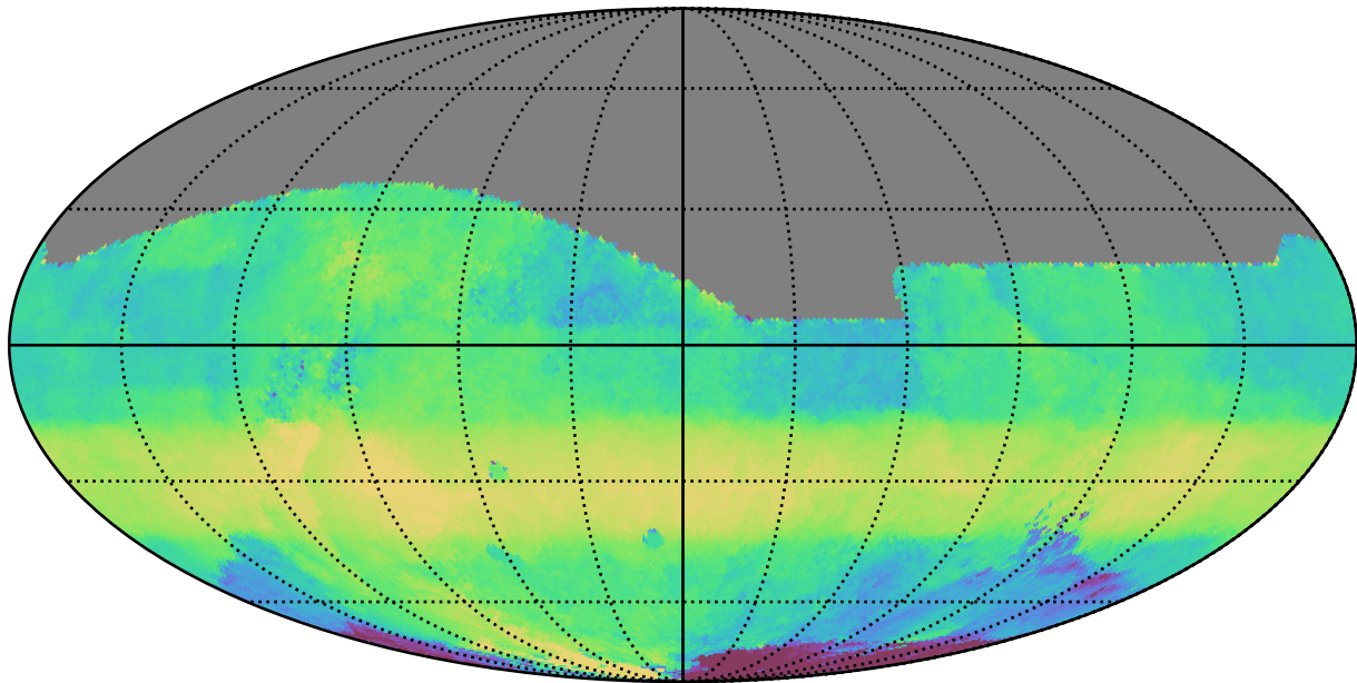
too_elab_r32_d3_ugrizy_v3.4_10yrs All sky r band: Median HA
