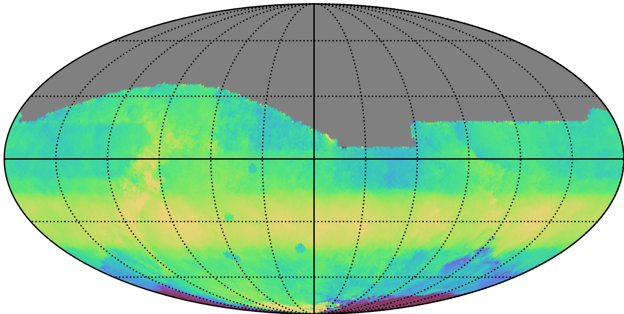
too_elab_r32_d3_ugrizy_v3.4_10yrs All sky i band: Median HA
