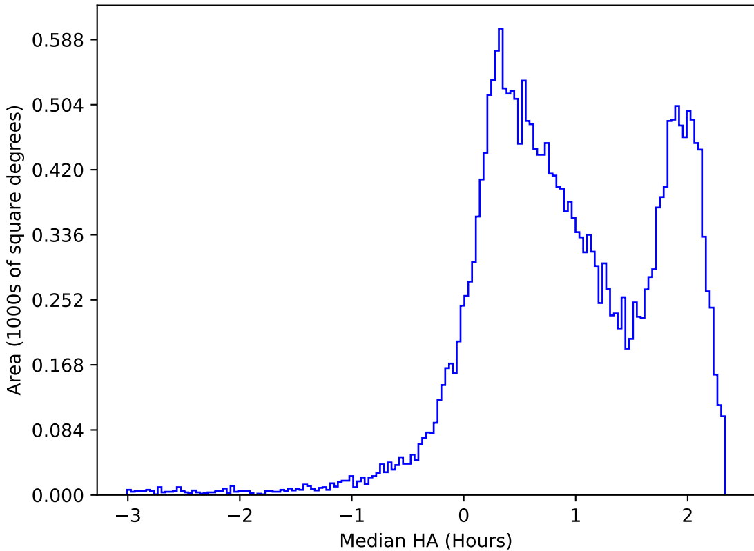
too_elab_r32_d3_ugrizy_v3.4_10yrs All sky i band: Median HA
