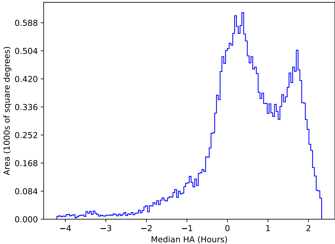
too_elab_r32_d3_ugrizy_v3.4_10yrs All sky g band: Median HA
