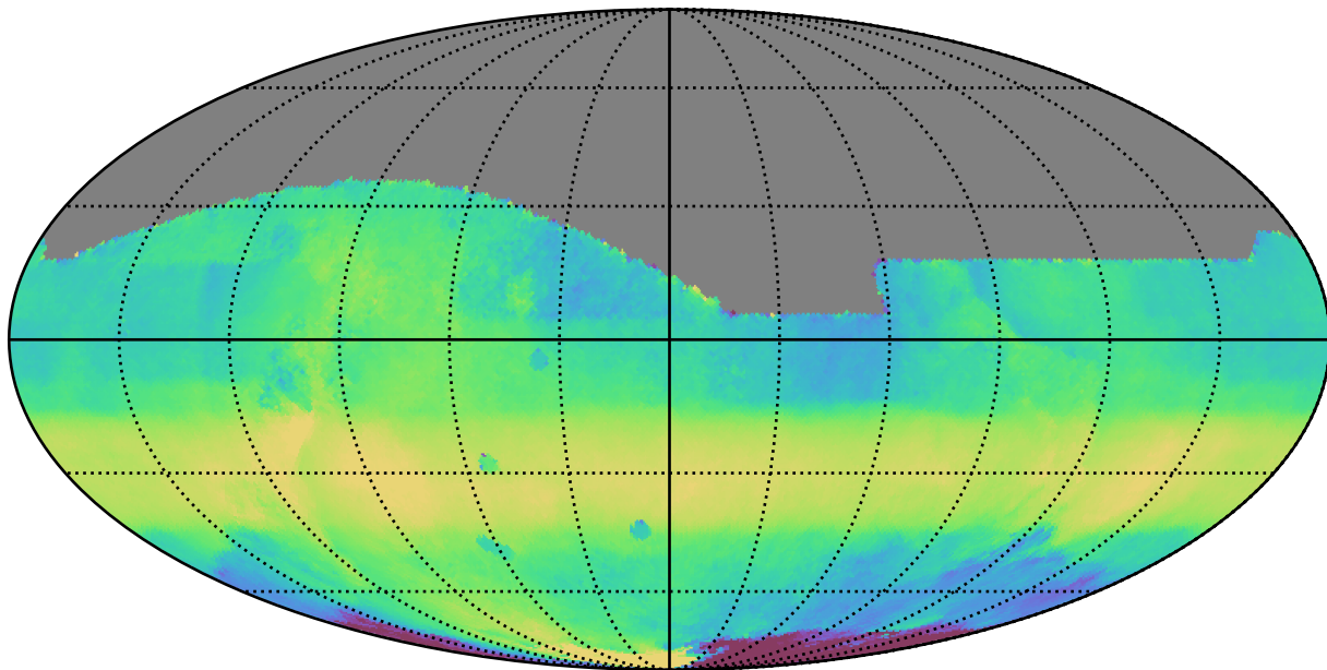
too_elab_r32_d3_ugrizy_v3.4_10yrs All sky all bands: Median HA
