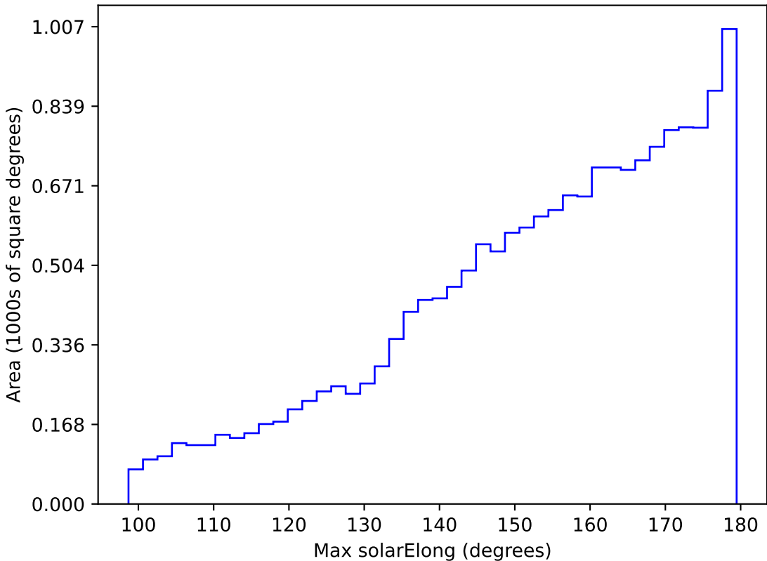
too_elab_r32_d3_ugrizy_v3.4_10yrs WFD z band: Max solarElong
