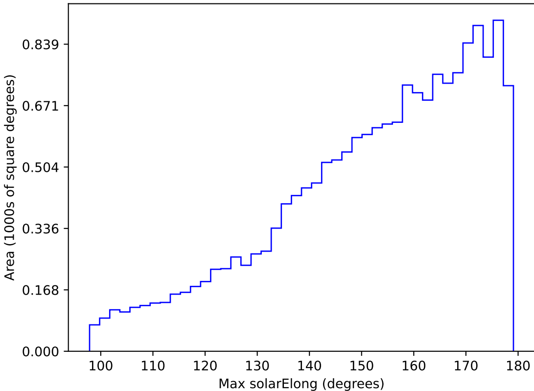
too_elab_r32_d3_ugrizy_v3.4_10yrs WFD u band: Max solarElong
