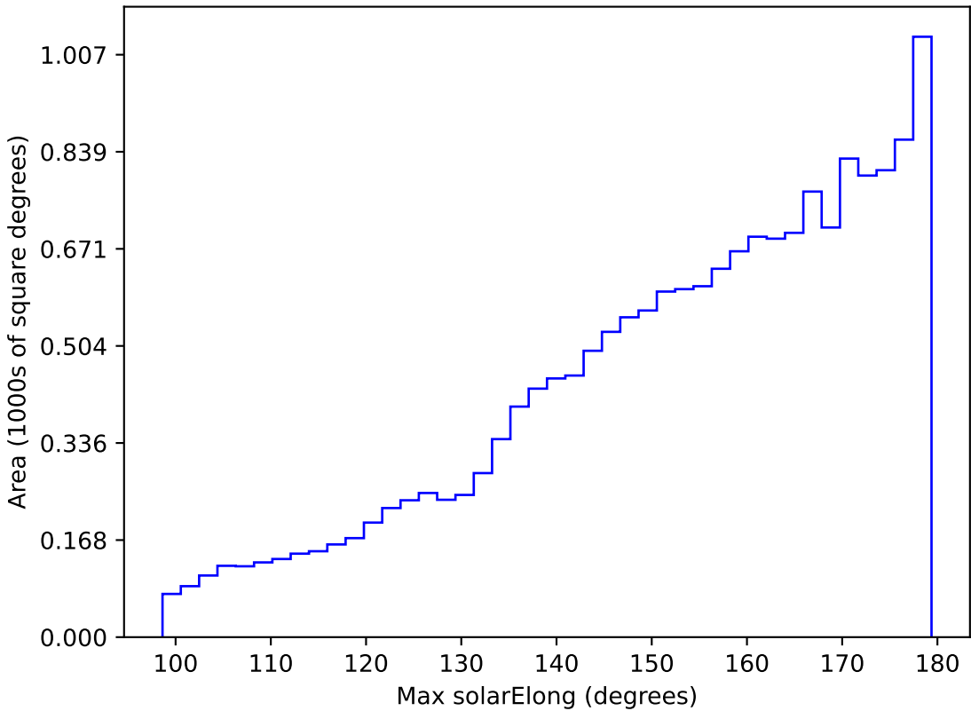
too_elab_r32_d3_ugrizy_v3.4_10yrs WFD r band: Max solarElong
