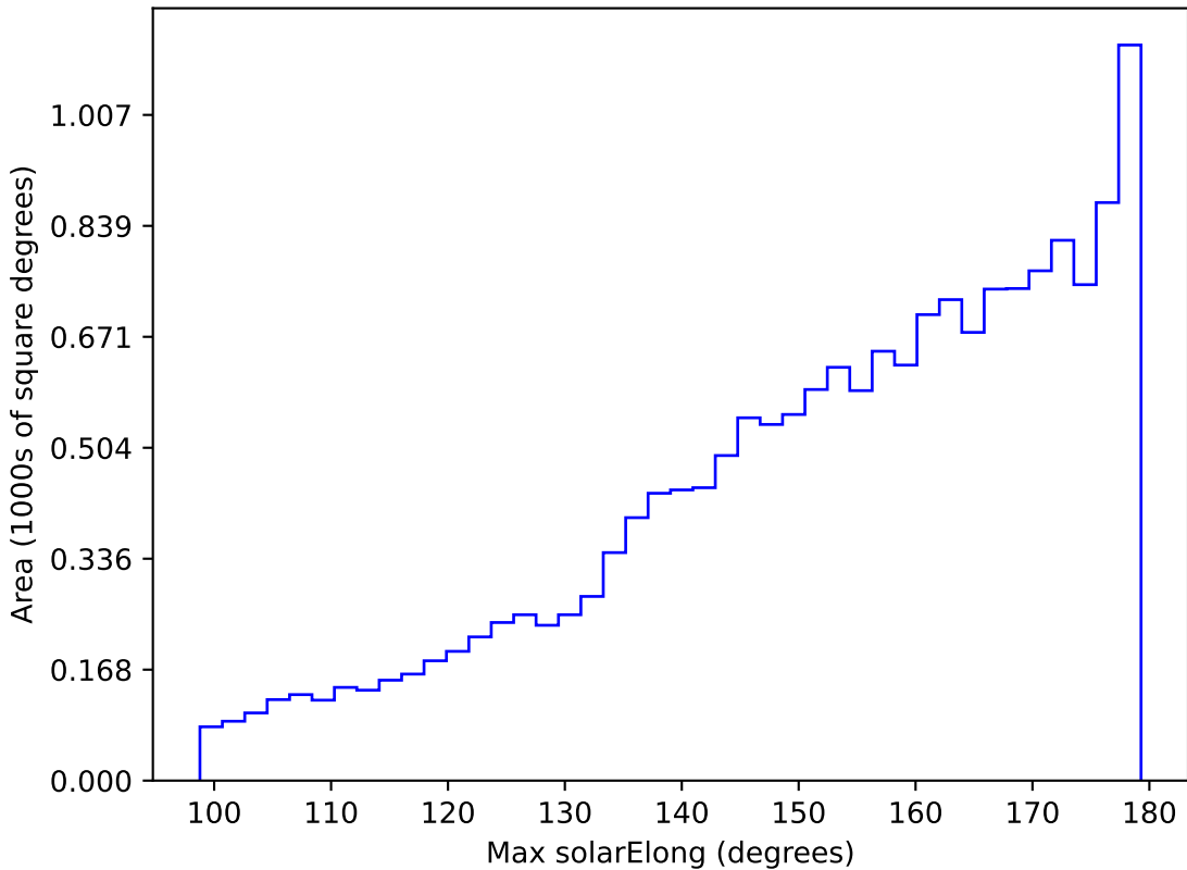
too_elab_r32_d3_ugrizy_v3.4_10yrs WFD i band: Max solarElong
