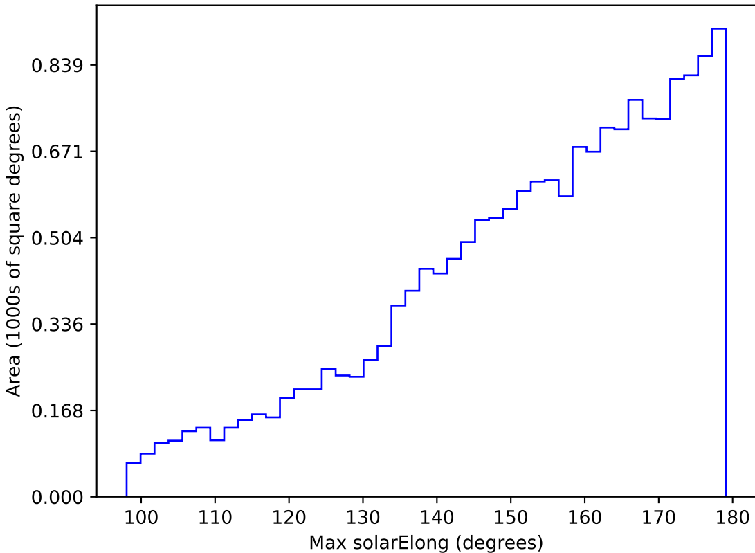
too_elab_r32_d3_ugrizy_v3.4_10yrs WFD g band: Max solarElong
