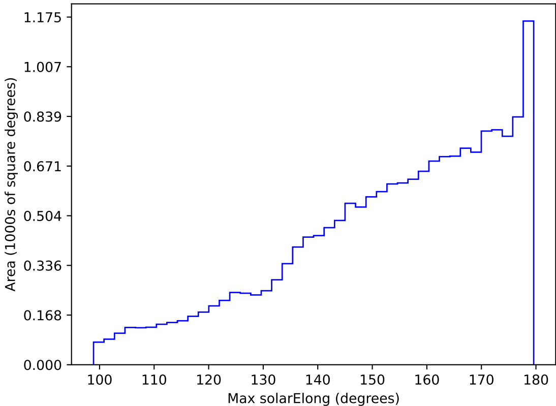
too_elab_r32_d3_ugrizy_v3.4_10yrs WFD all bands: Max solarElong
