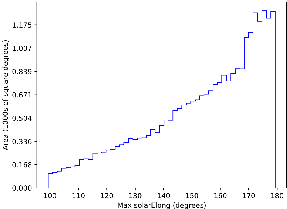
too_elab_r32_d3_ugrizy_v3.4_10yrs All sky z band: Max solarElong
