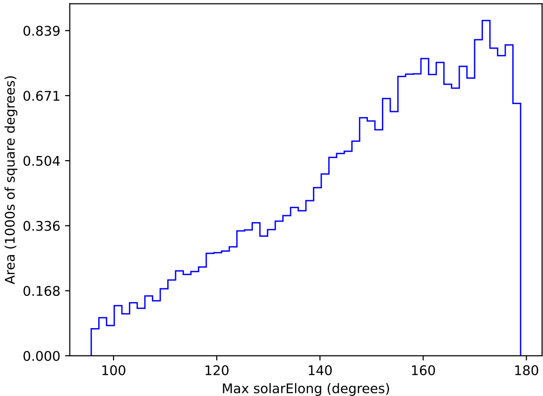
too_elab_r32_d3_ugrizy_v3.4_10yrs All sky u band: Max solarElong
