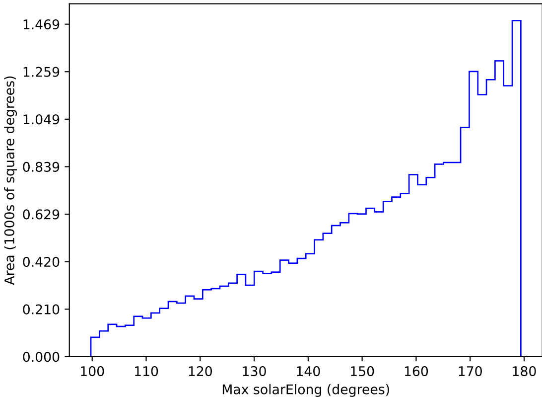
too_elab_r32_d3_ugrizy_v3.4_10yrs All sky r band: Max solarElong
