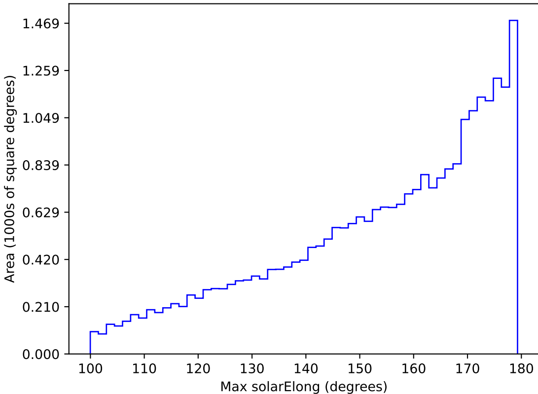
too_elab_r32_d3_ugrizy_v3.4_10yrs All sky i band: Max solarElong
