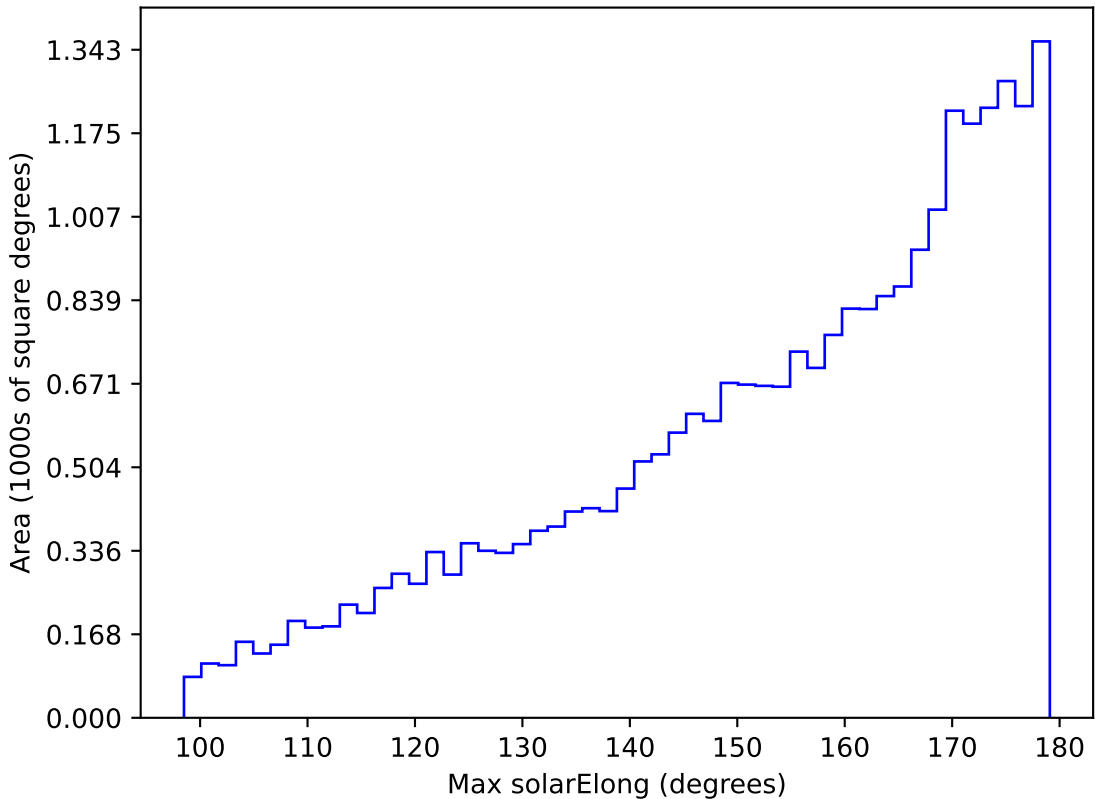
too_elab_r32_d3_ugrizy_v3.4_10yrs All sky g band: Max solarElong
