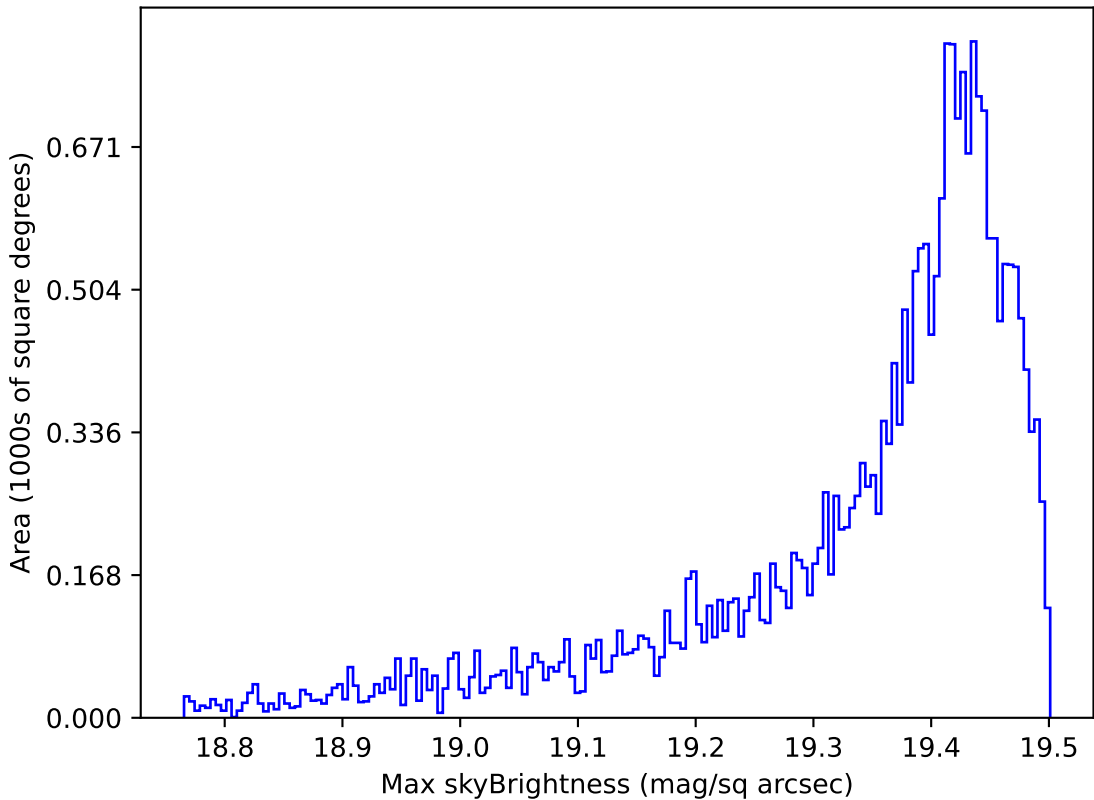
too_elab_r32_d3_ugrizy_v3.4_10yrs Yr 1 z band: Max skyBrightness
