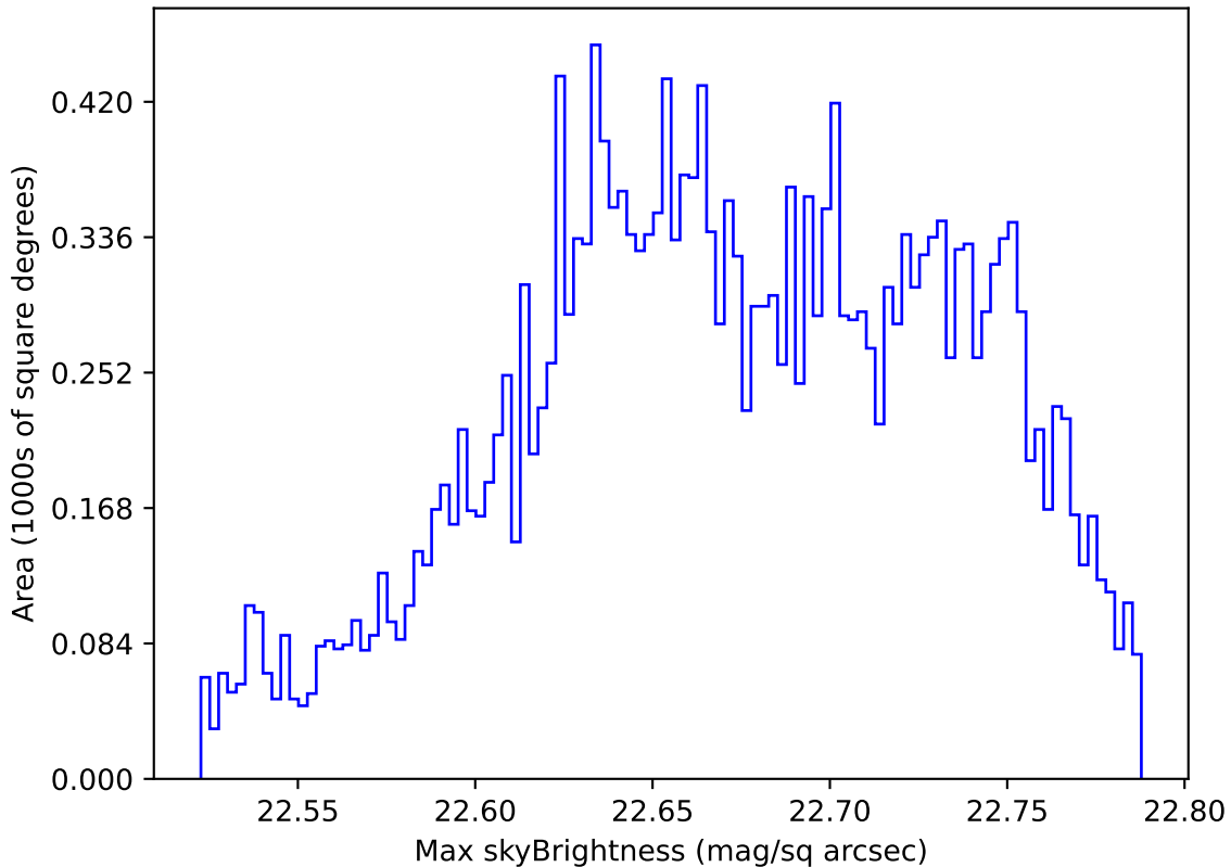
too_elab_r32_d3_ugrizy_v3.4_10yrs Yr 1 u band: Max skyBrightness
