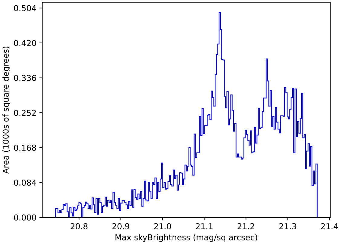
too_elab_r32_d3_ugrizy_v3.4_10yrs Yr 1 r band: Max skyBrightness
