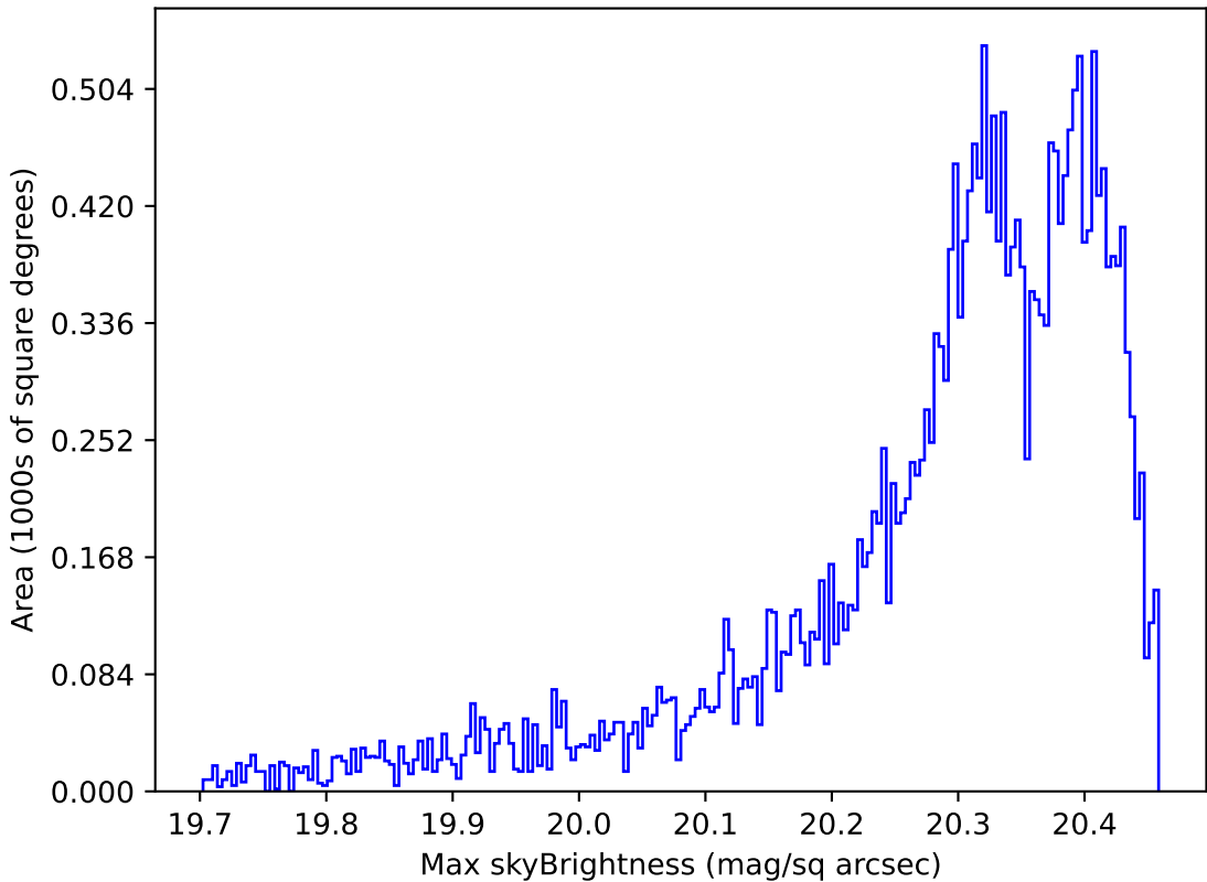
too_elab_r32_d3_ugrizy_v3.4_10yrs Yr 1 i band: Max skyBrightness
