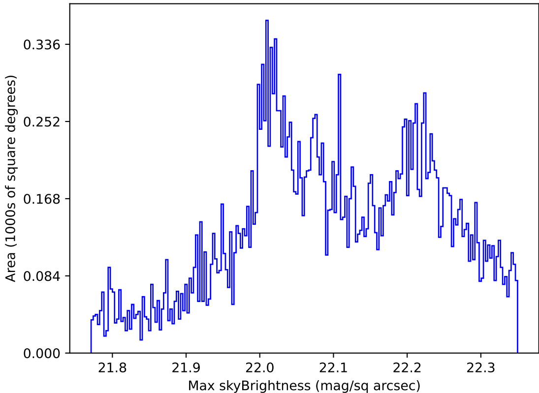
too_elab_r32_d3_ugrizy_v3.4_10yrs Yr 1 g band: Max skyBrightness
