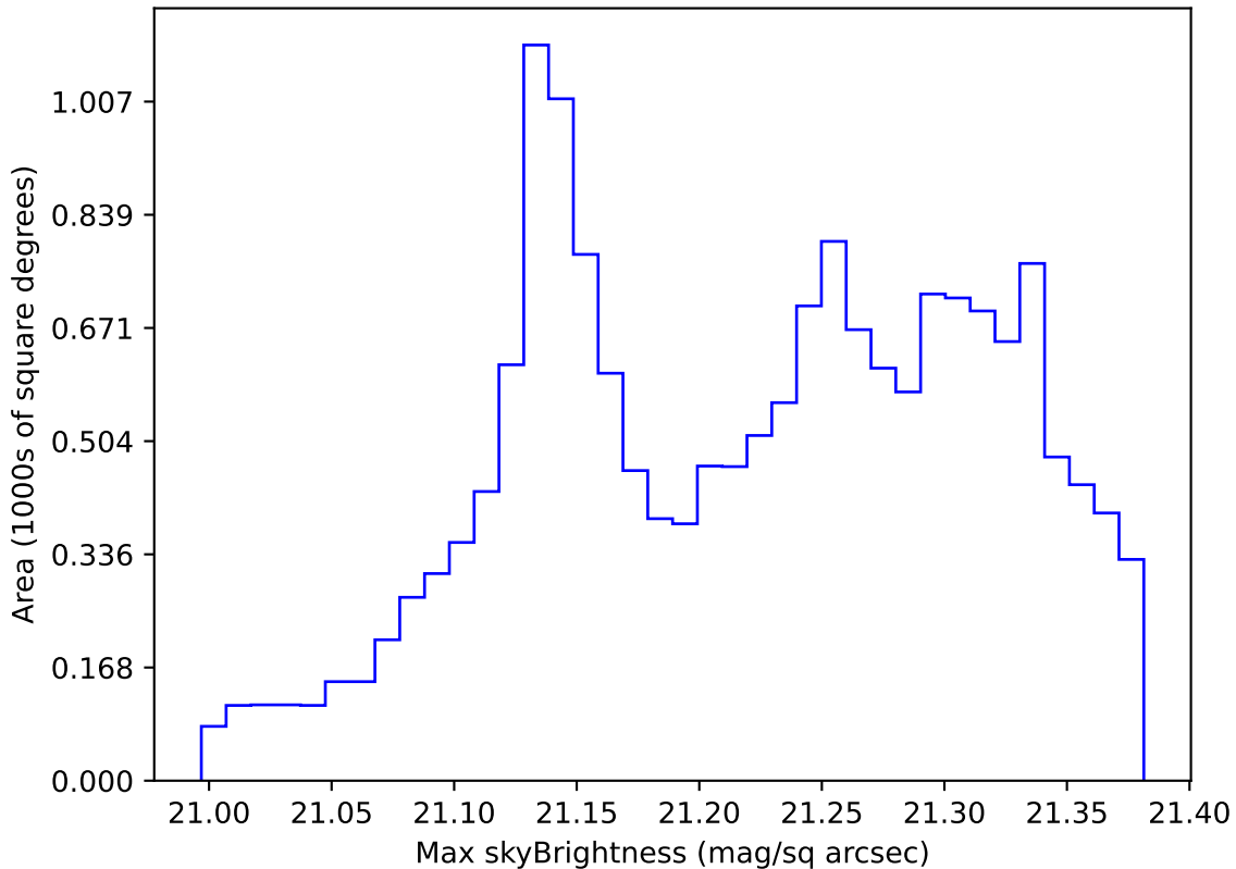
too_elab_r32_d3_ugrizy_v3.4_10yrs WFD r band: Max skyBrightness
