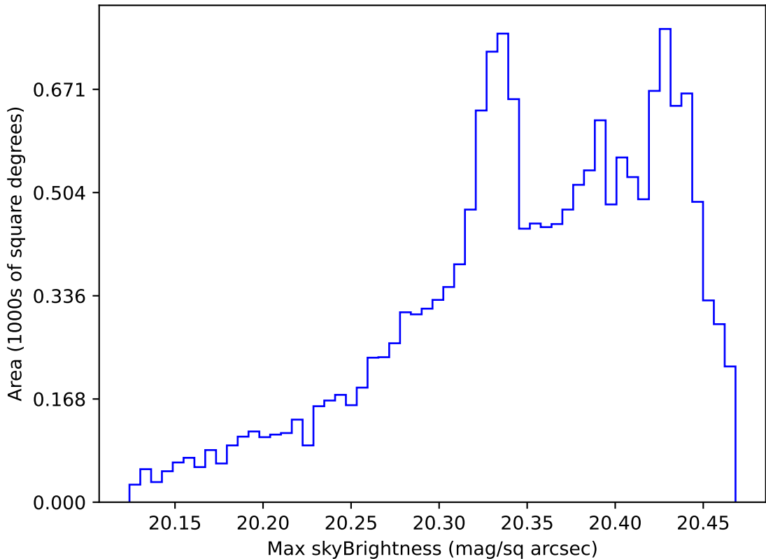
too_elab_r32_d3_ugrizy_v3.4_10yrs WFD i band: Max skyBrightness
