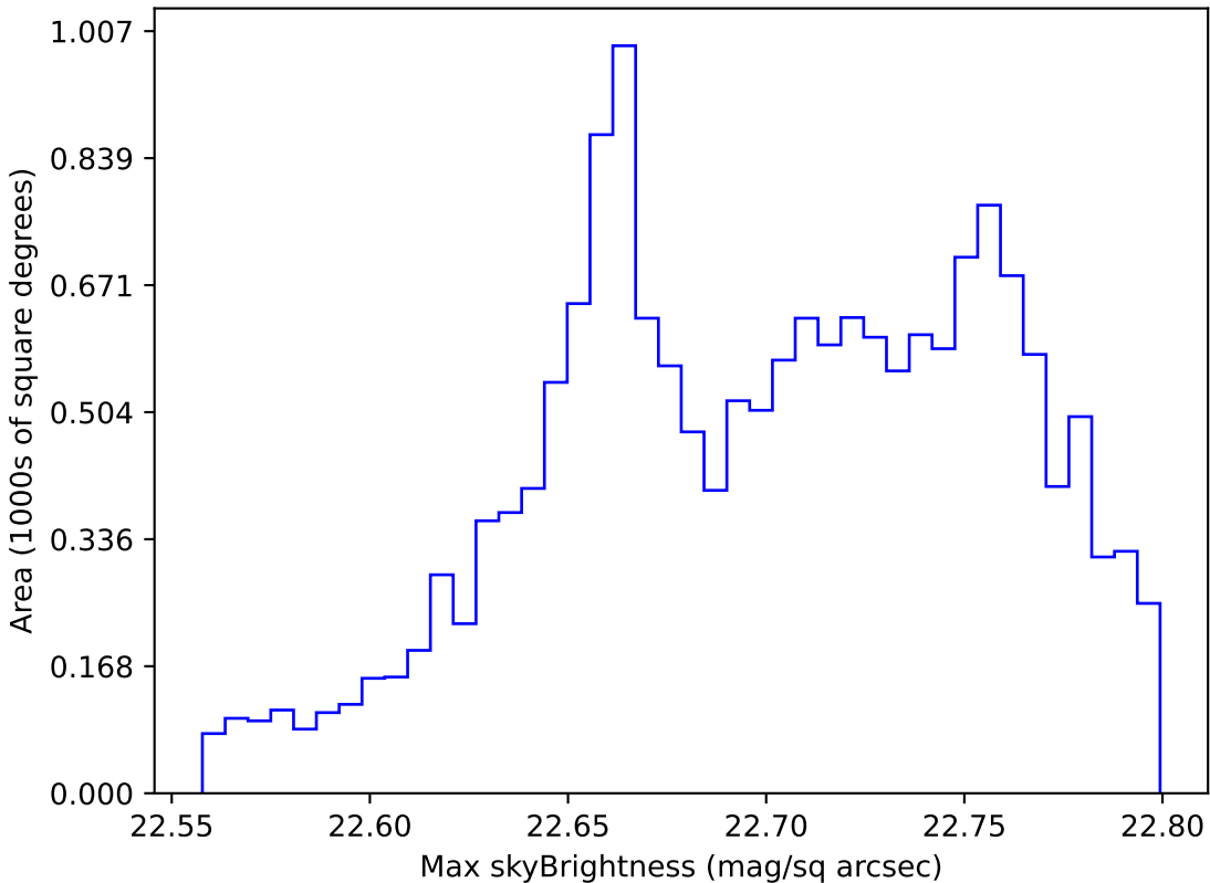
too_elab_r32_d3_ugrizy_v3.4_10yrs WFD all bands: Max skyBrightness
