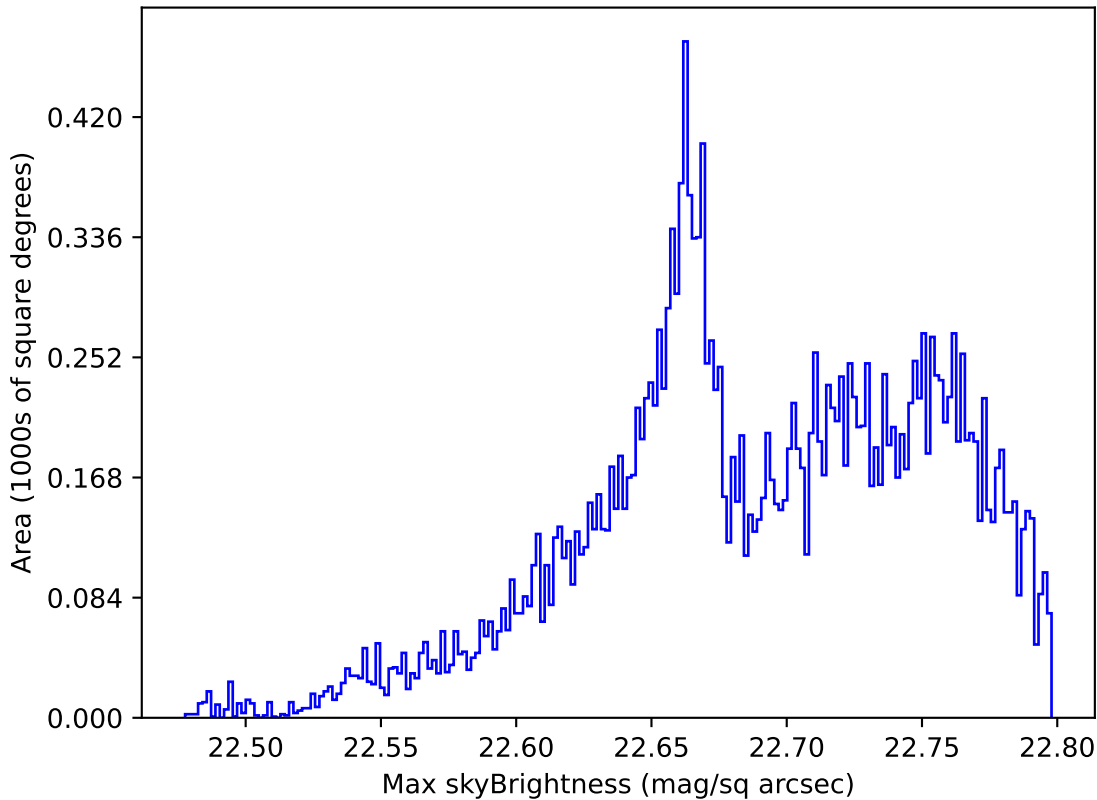
too_elab_r32_d3_ugrizy_v3.4_10yrs All sky u band: Max skyBrightness
