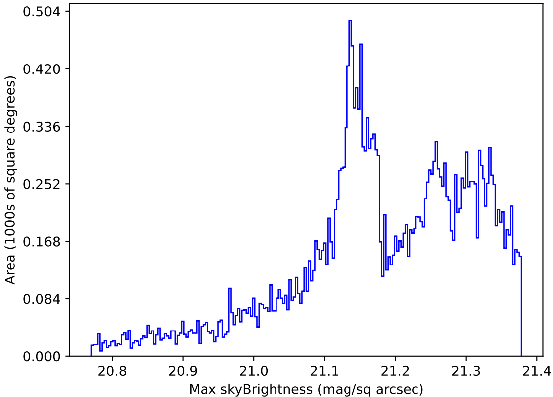
too_elab_r32_d3_ugrizy_v3.4_10yrs All sky r band: Max skyBrightness
