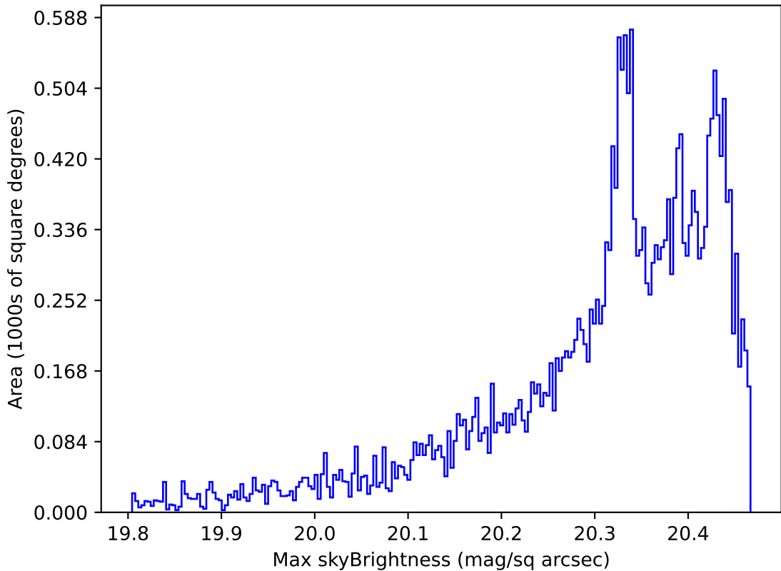
too_elab_r32_d3_ugrizy_v3.4_10yrs All sky i band: Max skyBrightness
