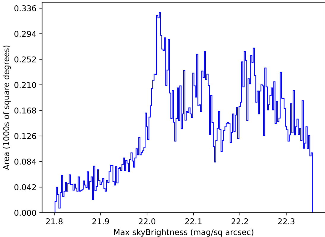
too_elab_r32_d3_ugrizy_v3.4_10yrs All sky g band: Max skyBrightness
