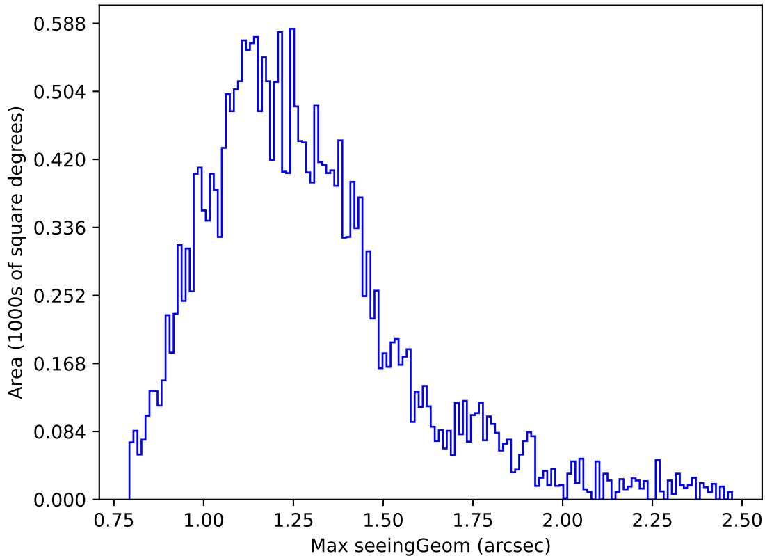
too_elab_r32_d3_ugrizy_v3.4_10yrs Yr 1 z band: Max seeingGeom
