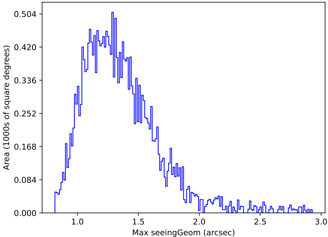
too_elab_r32_d3_uigrzy_v3.4_10yrs Yr 1 u band: Max seeingGeom
