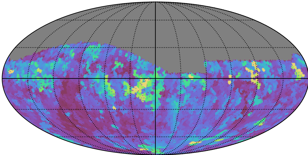
too_elab_r32_d3_ugrizy_v3.4_10yrs Yr 1 z band: Max seeingEff
