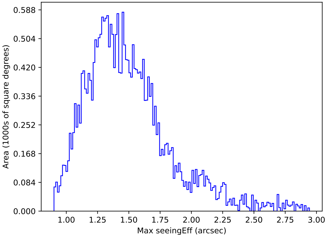
too_elab_r32_d3_ugrizy_v3.4_10yrs Yr 1 z band: Max seeingEff
