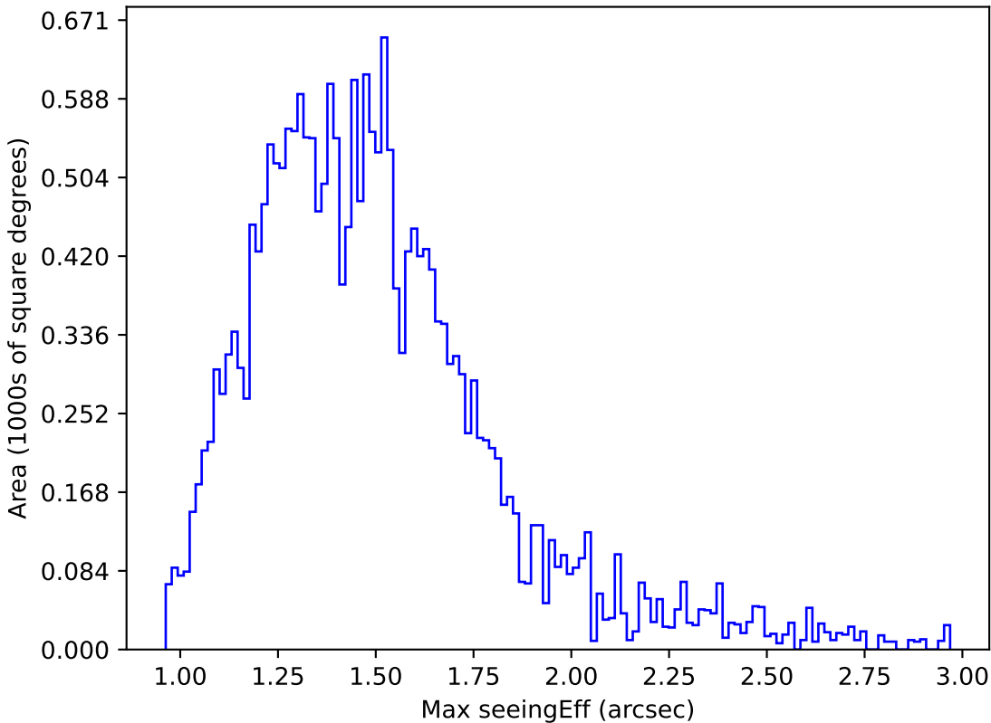
too_elab_r32_d3_ugrizy_v3.4_10yrs Yr 1 y band: Max seeingEff
