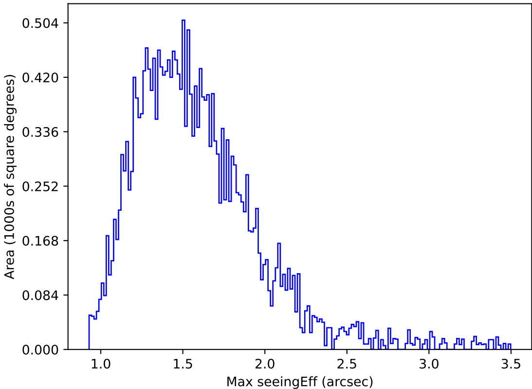
too_elab_r32_d3_ugrizy_v3.4_10yrs Yr 1 u band: Max seeingEff
