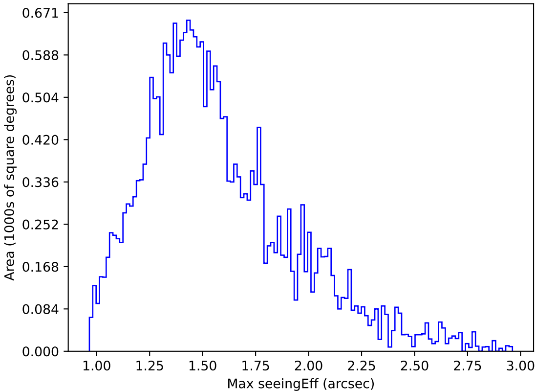
too_elab_r32_d3_ugrizy_v3.4_10yrs Yr 1 r band: Max seeingEff
