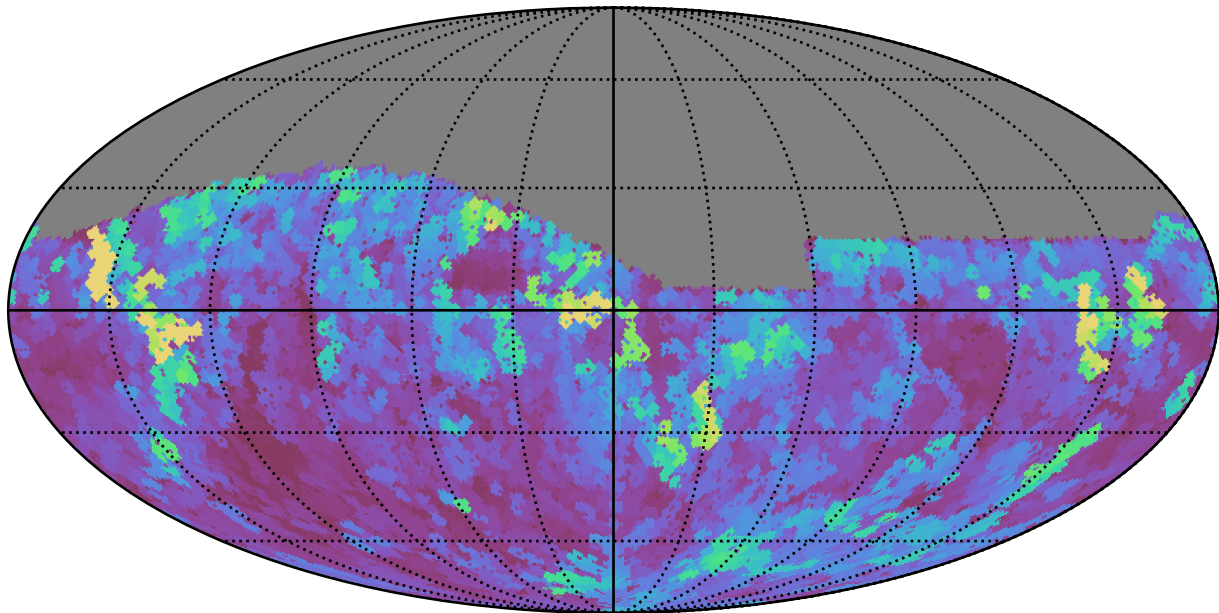
too_elab_r32_d3_ugrizy_v3.4_10yrs Yr 1 i band: Max seeingEff
