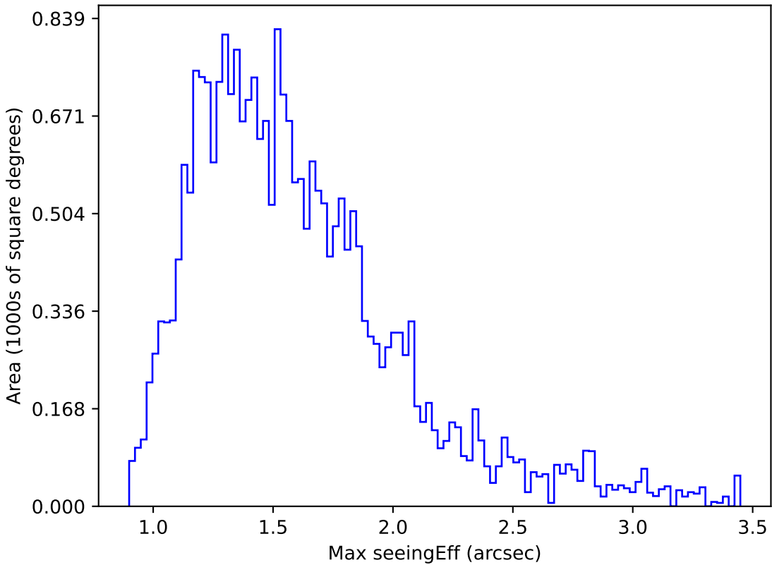
too_elab_r32_d3_ugrizy_v3.4_10yrs Yr 1 g band: Max seeingEff
