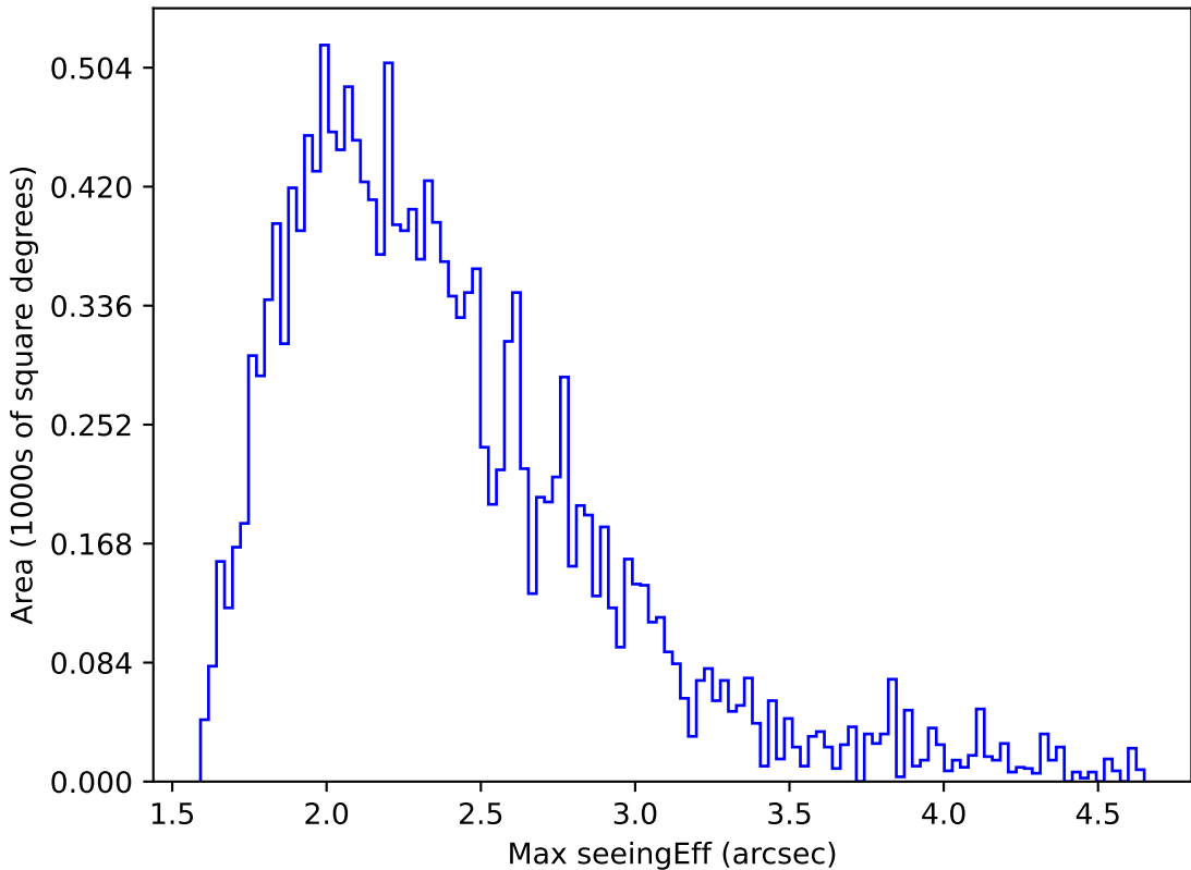
too_elab_r32_d3_ugrizy_v3.4_10yrs WFD y band: Max seeingEff
