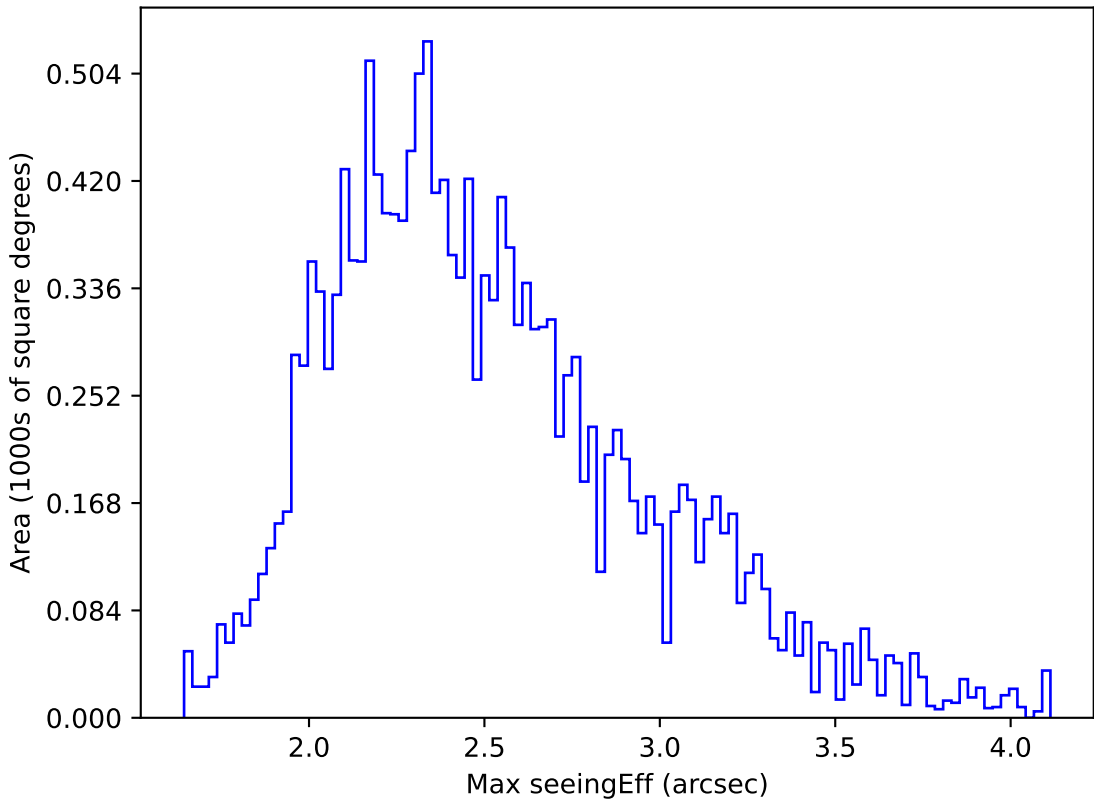
too_elab_r32_d3_ugrizy_v3.4_10yrs WFD u band: Max seeingEff
